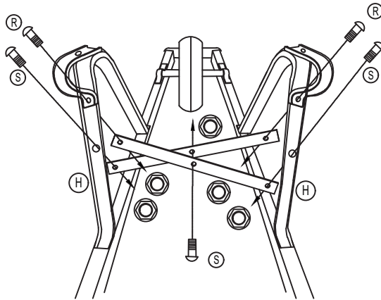
LEG BRACE ASSEMBLY
