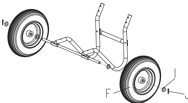
WHEEL ASSEMBLY
