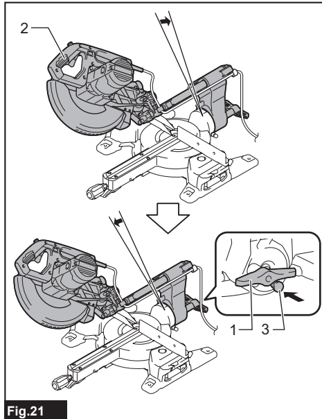
► 1. Lever 2. Handle 3. Releasing button
